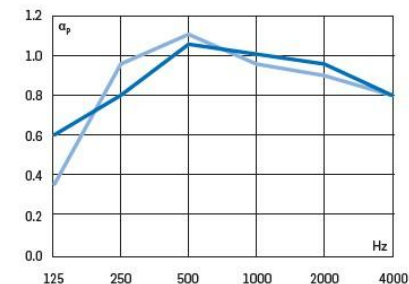
BASWA Phon Fine 70mm
