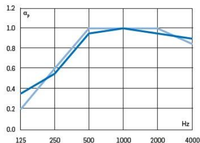
BASWA Phon Fine 40mm
