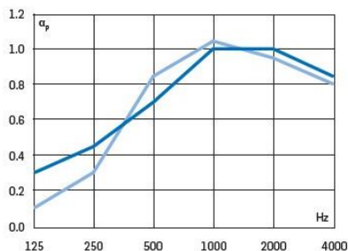
BASWA Phon Fine 30mm
