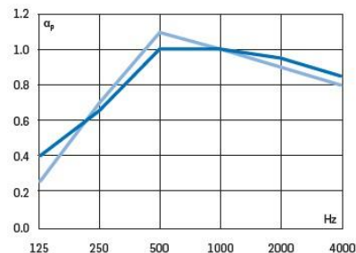
BASWA Phon Fine 50mm
