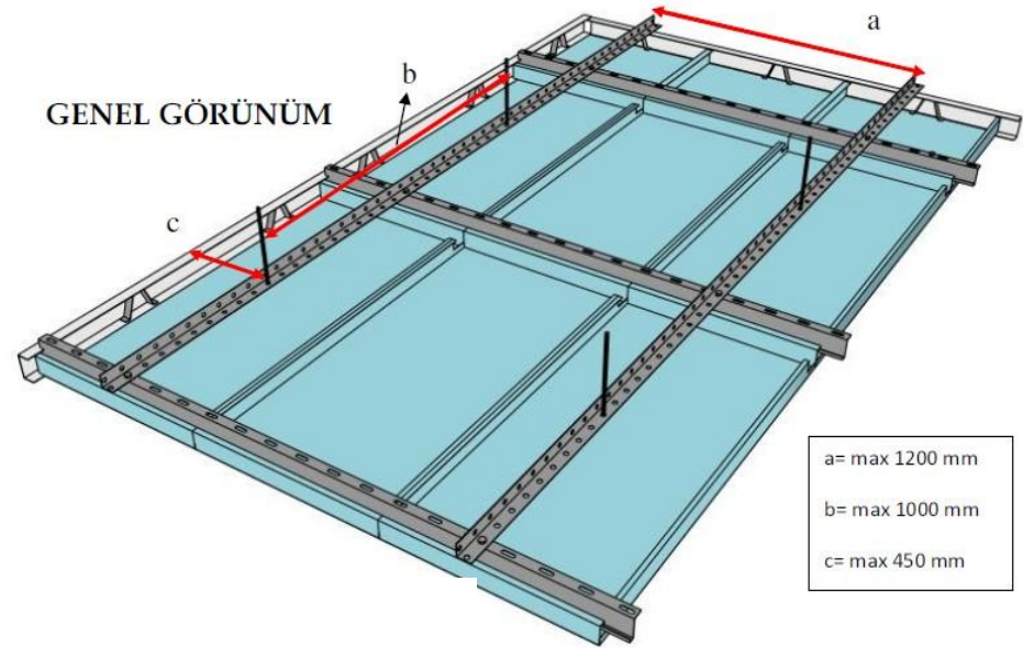
HOOK-ON PLANK SİSTEM
